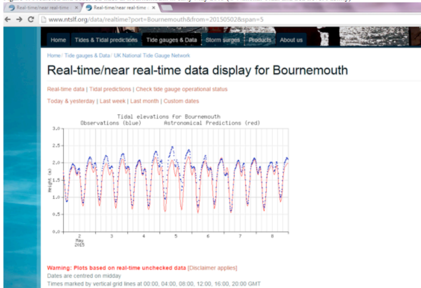
Figure 1. Predicted and observed tides at Bournemouth in early May 2015 (© National Tidal and Sea Level Facility)
